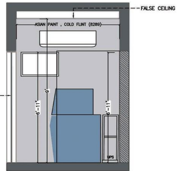
03 1:50 INTERNAL ELEVATION-03 XIE-0101
