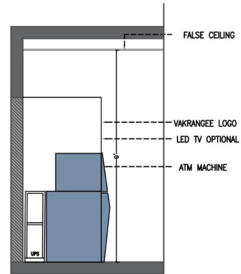
SECTIONAL ELEVATION 4
