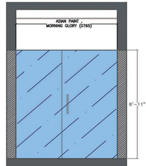
05 1:50 INTERNAL ELEVATION-05 XIE-0101
