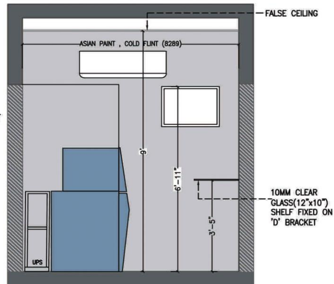
03 1:50 INTERNAL ELEVATION - 03 XIE-0101
