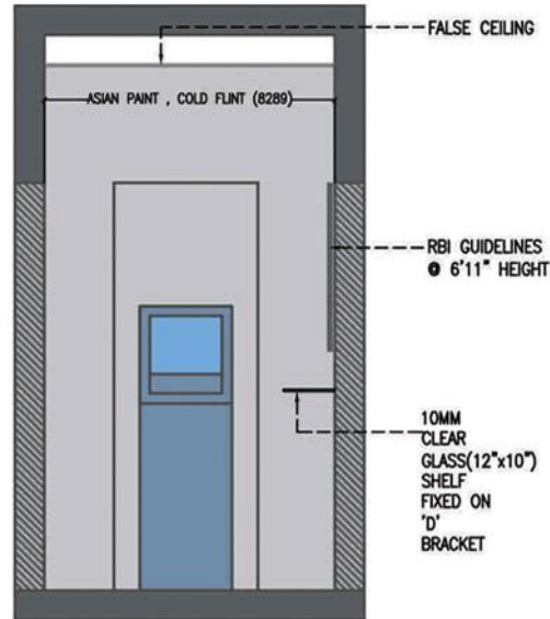
03 XIE-0101 1:50 INTERNAL ELEVATION - 03 GROUND FLOOR
