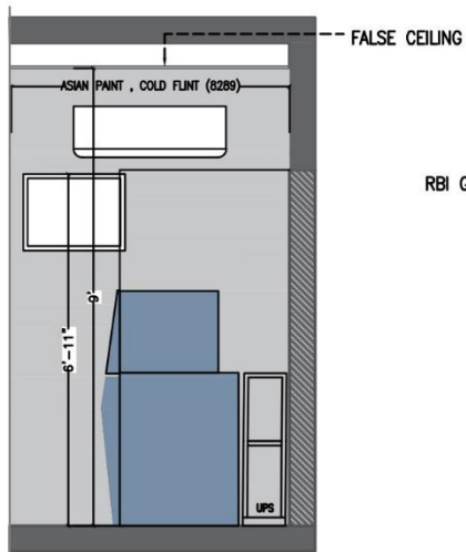
SECTIONAL ELEVATION 3
