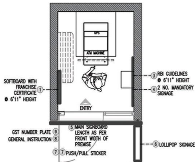
01 XIE-0101 1:20 GENERAL ARRANGEMENT PLAN GROUND FLOOR
