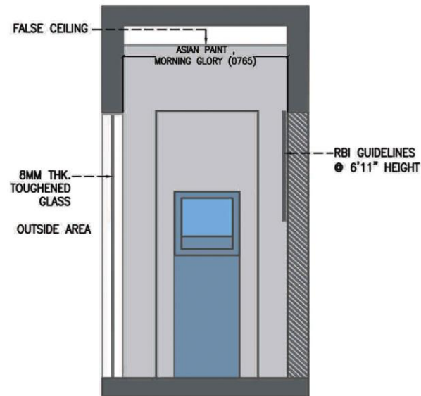
02 1:50 INTERNAL ELEVATION - 02 XIE-0101
