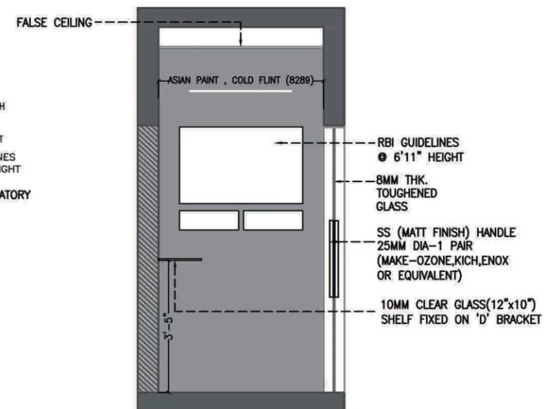
05 1:50 INTERNAL ELEVATION - 05 XIE-0101
