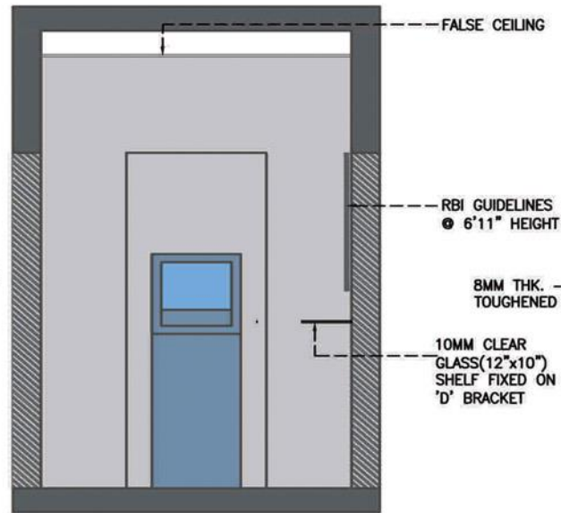
02 1:50 INTERNAL ELEVATION-02 XIE-0101
