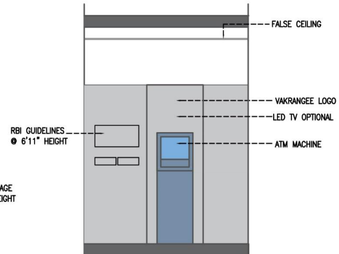
FRONT ELEVATION 2
