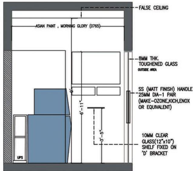
02 XIE-0101 1:50 INTERNAL ELEVATION - 02 GROUND FLOOR
