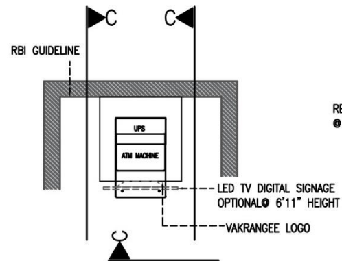
PLAN 1
