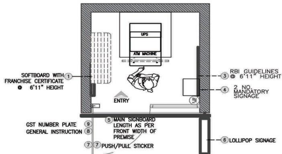
01 1:20 GENERAL ARRANGEMENT PLAN XIE-0101
