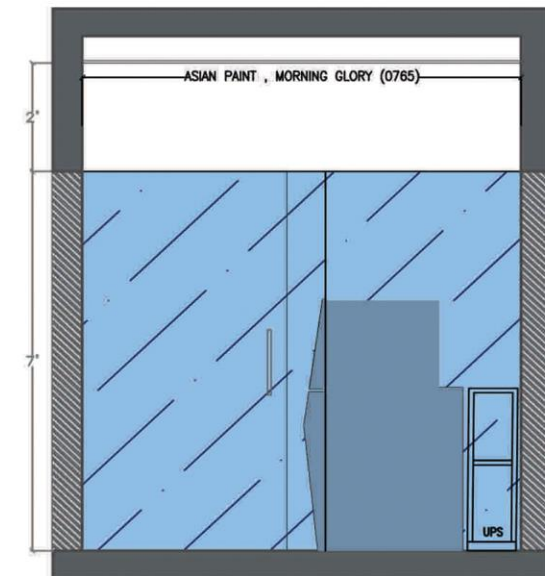
04 1:50 INTERNAL ELEVATION - 04 XIE-0101
