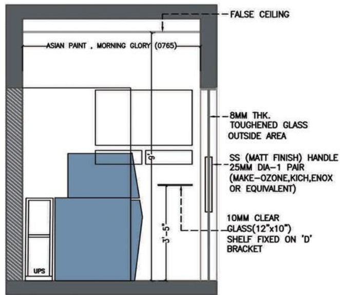
04 1:50 INTERNAL ELEVATION-04 XIE-0101
