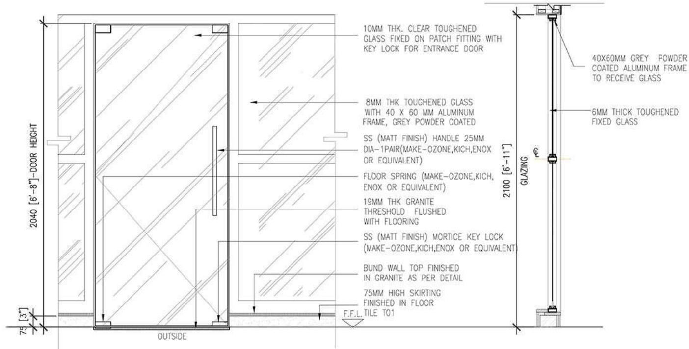
05 1:20 ELEVATION AND SECTION D02-0102 MAIN ENTRANCE- OPTION 3
