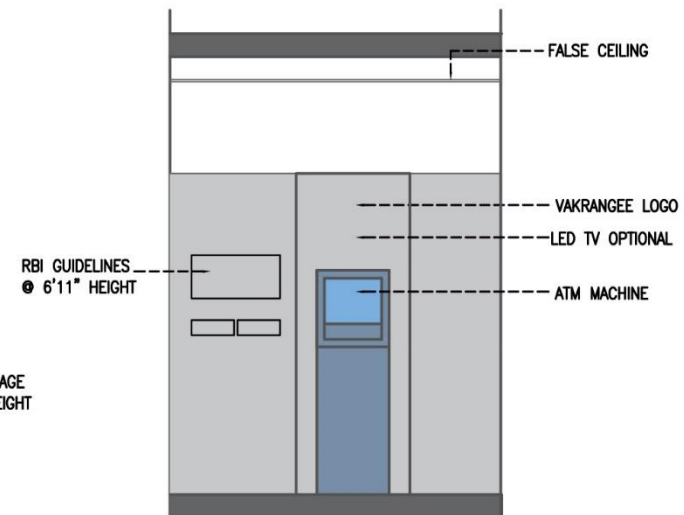
FRONT ELEVATION 2
