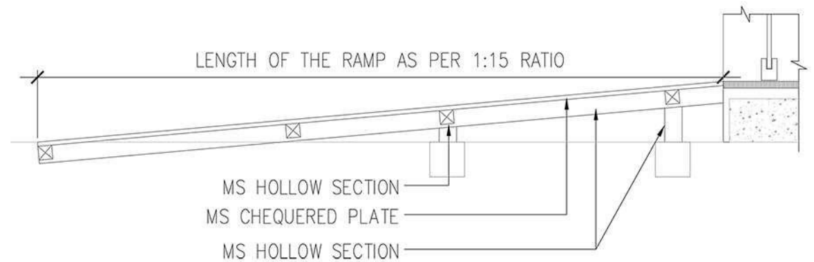
06 D01-0104 1:20 SECTION - OPTION 2 ENTRANCE RAMP
