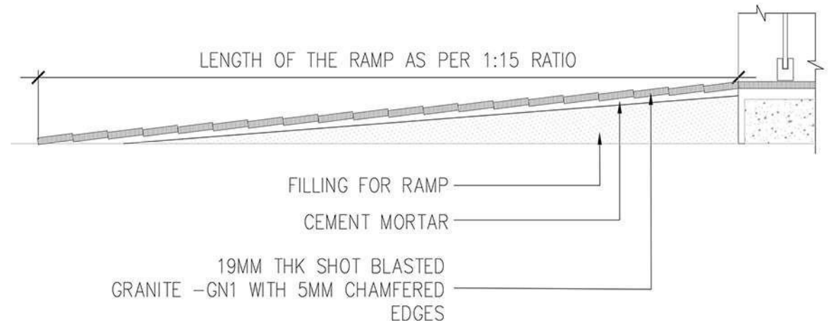
06 D01-0106 1:20 SECTION - OPTION 1 ENTRANCE RAMP
