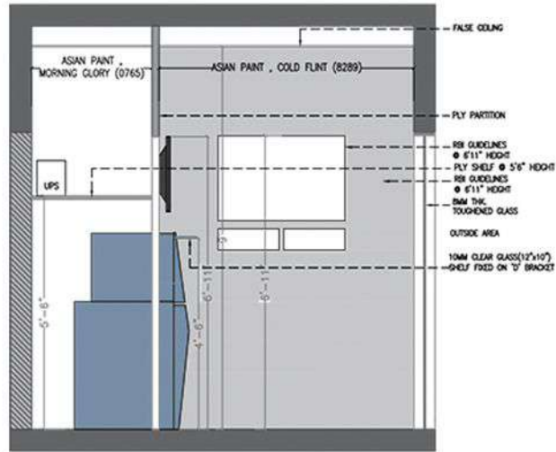
02 XIE-0101 1:50 INTERNAL ELEVATION - 02 GROUND FLOOR
