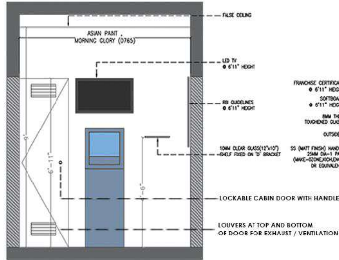
02 1:50 INTERNAL ELEVATION-02 XIE-0101
