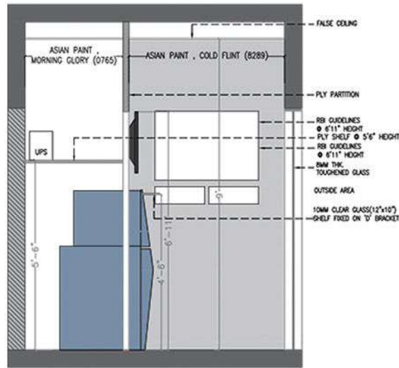
04 1:50 INTERNAL ELEVATION-04 XIE-0101
