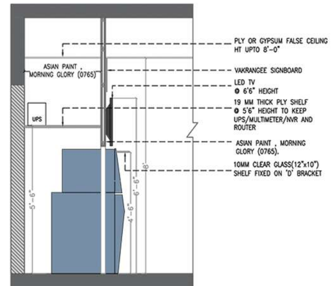
SECTIONAL ELEVATION 4
