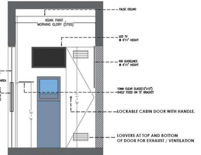
04 XIE-0101 1:50 INTERNAL ELEVATION - 04
