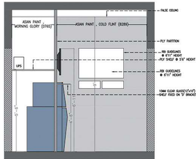
03 XIE-0101 1:50 INTERNAL ELEVATION - 03
