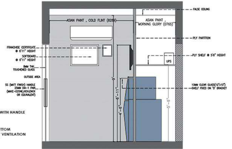
04 XIE-0101 1:50 INTERNAL ELEVATION - 04 GROUND FLOOR
