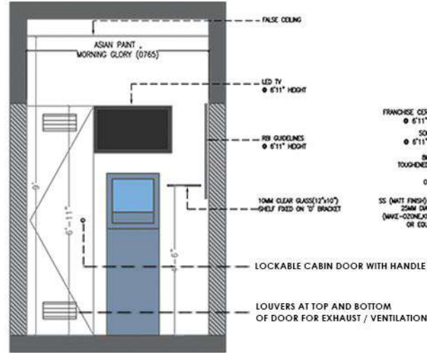
03 XIE-0101 1:50 INTERNAL ELEVATION - 03 GROUND FLOOR
