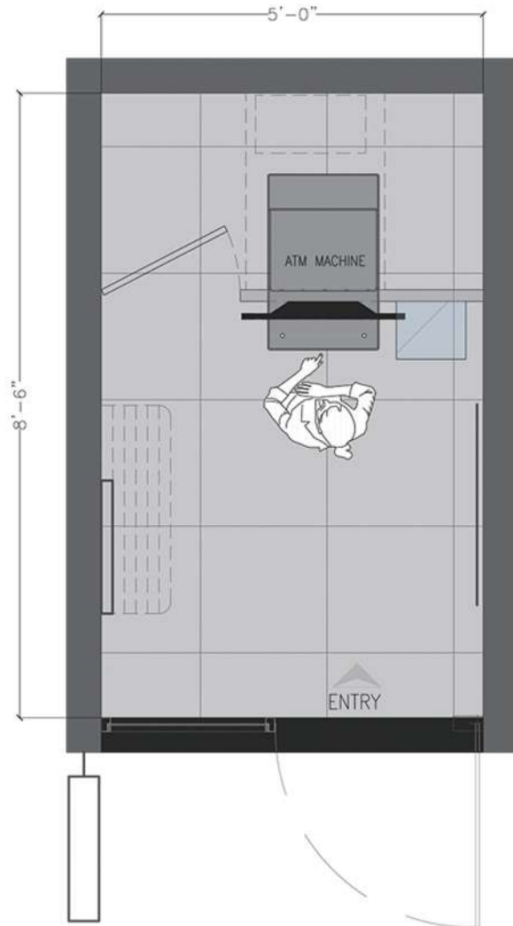
Top View
