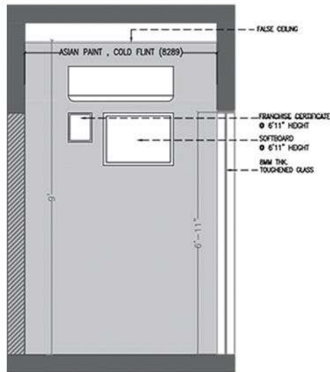
02 XIE-0101 1:50 INTERNAL ELEVATION - 02
