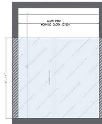
05 1:50 INTERNAL ELEVATION-05 XIE-0101
