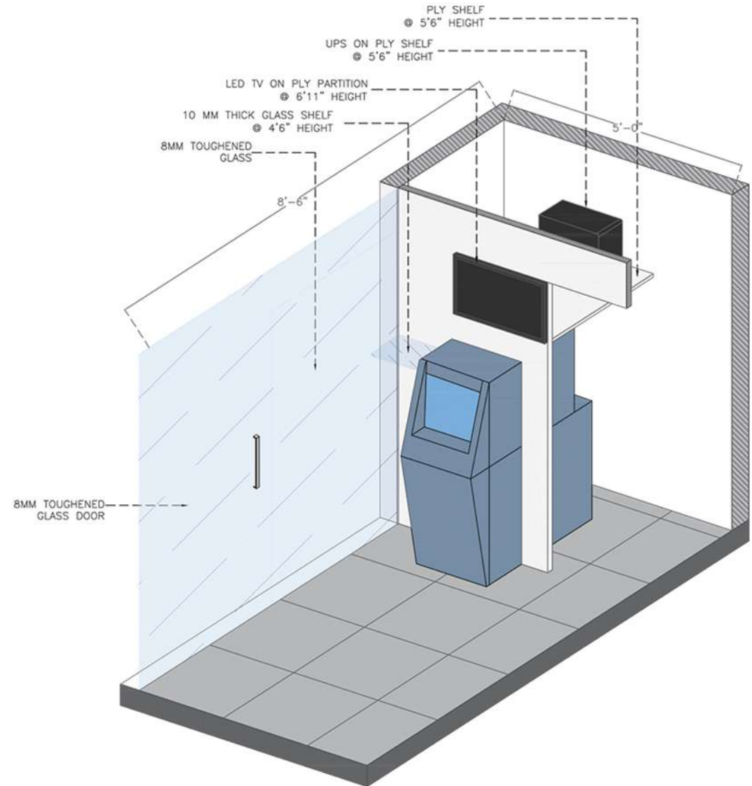
Isometric View
