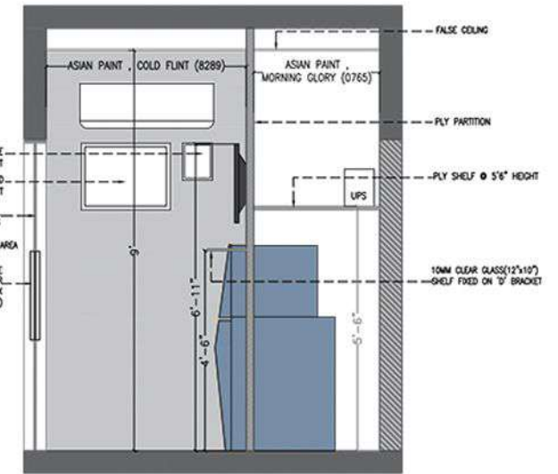
03 1:50 INTERNAL ELEVATION-03 XIE-0101
