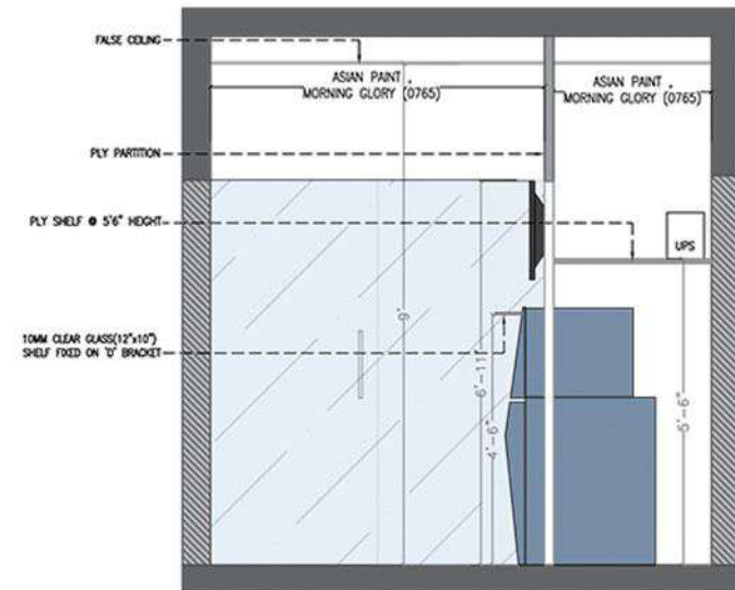
05 XIE-0101 1:50 INTERNAL ELEVATION - 05
