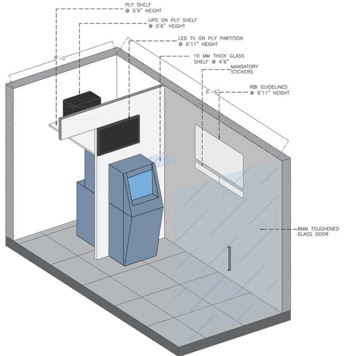
Isometric View
