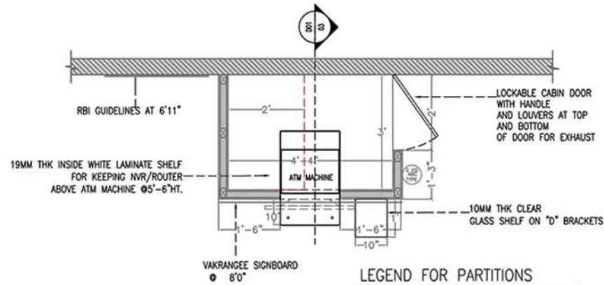
LEGEND FOR PARTITIONS
