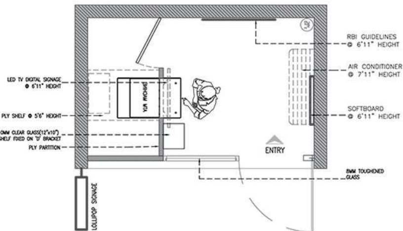
01 XIE-0101 1:20 GENERAL ARRANGEMENT PLAN
